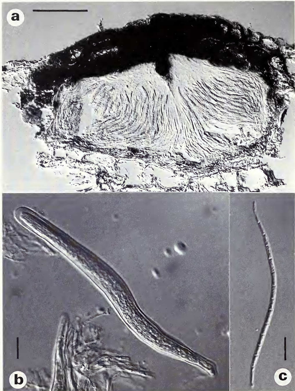
Fig. 39 Celothelium stenobelum (Nyl.) Aguirre (H-NYL 640-holotype) (a) Vertical section of ascoma; scale = 100 \mu\text{m} ; (b) Ascus and ascospores; (c) Ascospore; scale = 10 \mu\text{m} .
